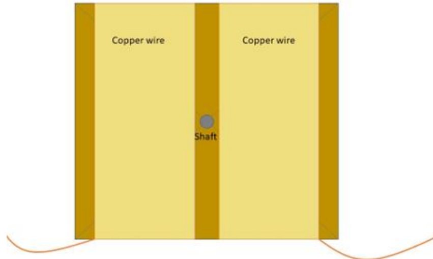
Figure 6. Neatly wind the copper wire around the frame, ensuring you leave a "tail" at each end to connect the ammeter to.
